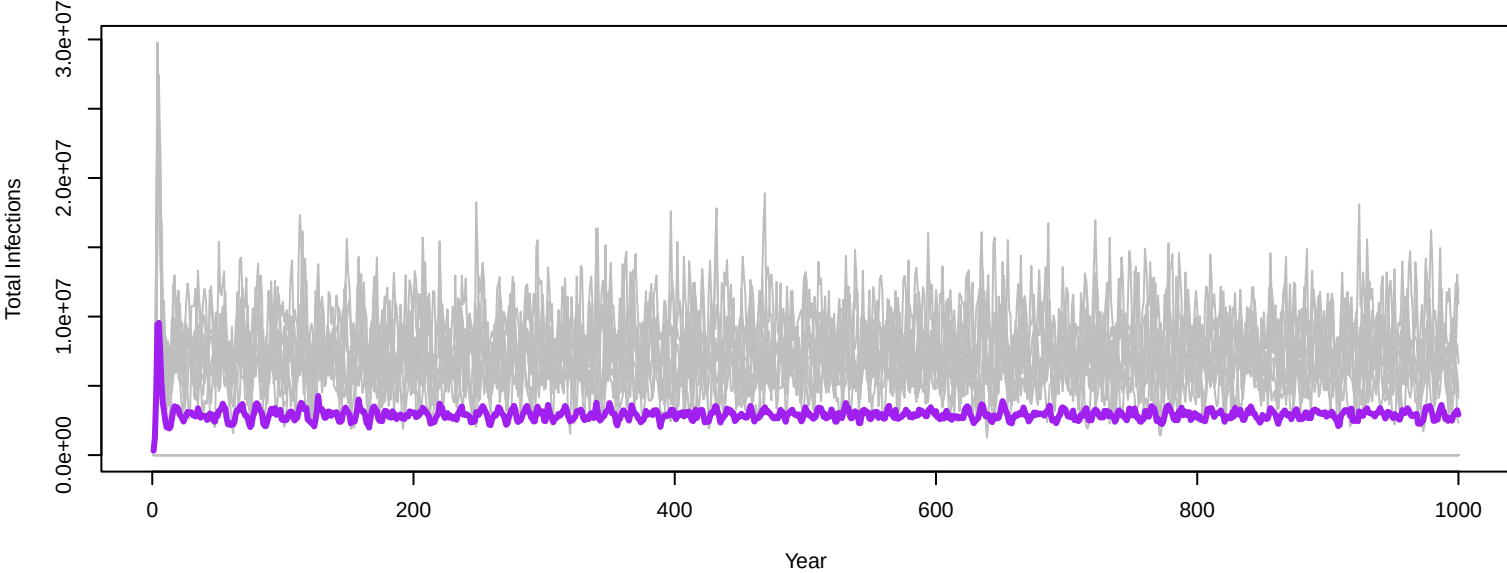
Total Infections Over Time
